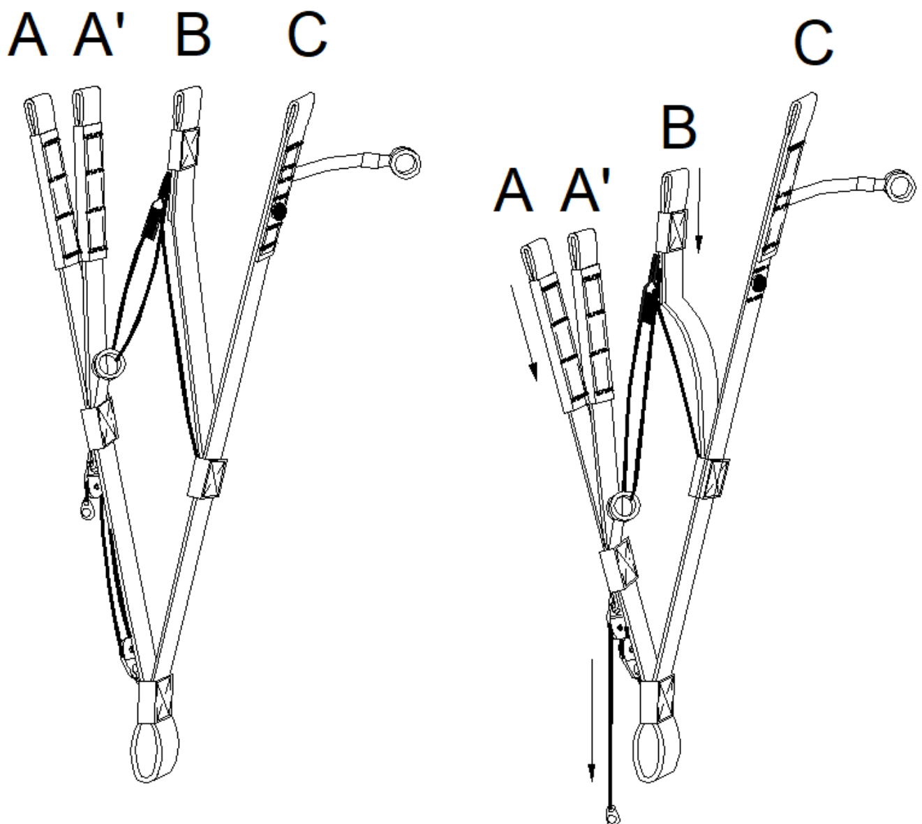
Figure: Bandit2 riser (standard)
